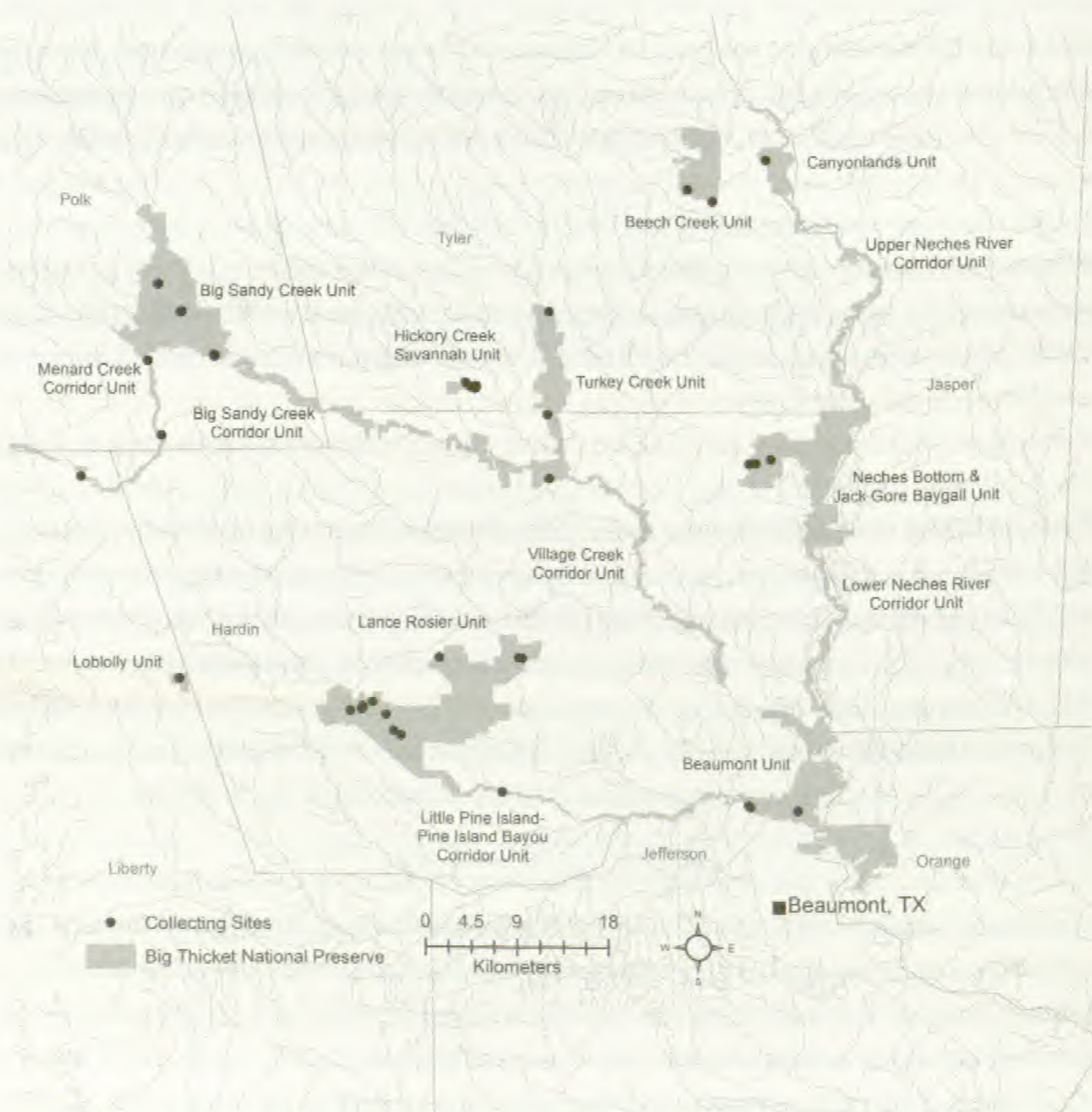
FIG. 1. A map of collecting localities within the Big Thicket National Preserve in eastern Texas.
